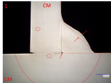
Figure 6. Macroscopic view of specimen 1
