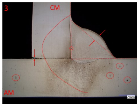
Figure 8. Macroscopic view of specimen 3
