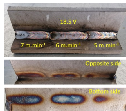
Figure 3. Welds of combinations 1, 3 and 5 from Tab. 8
